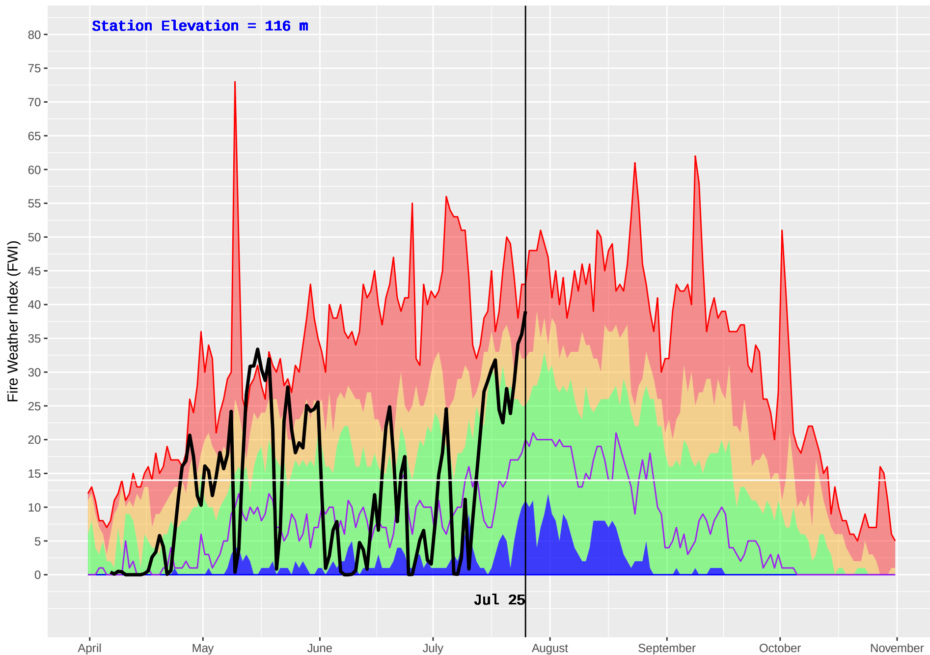
SCAR CREEK (82) : Historical (1982–2016) and Current (2018) Noon Fire Weather Index (FWI)
